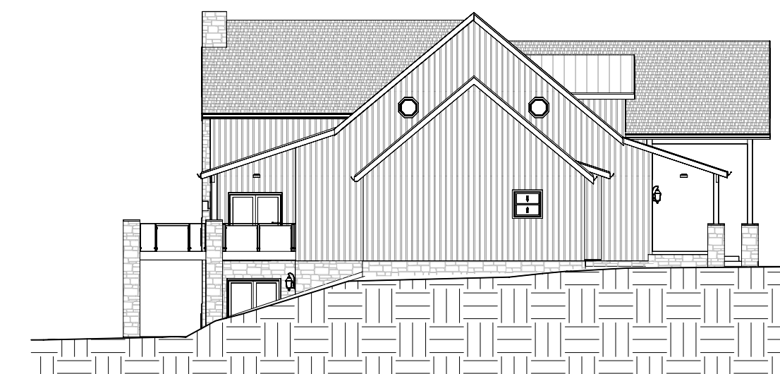
⑦ West 1/16" = 1'-0"
