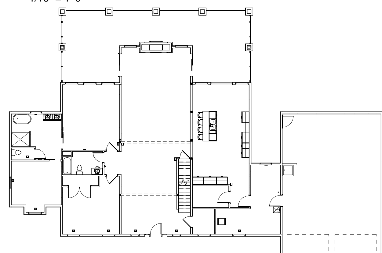
① First Floor 1/16" = 1'-0"
