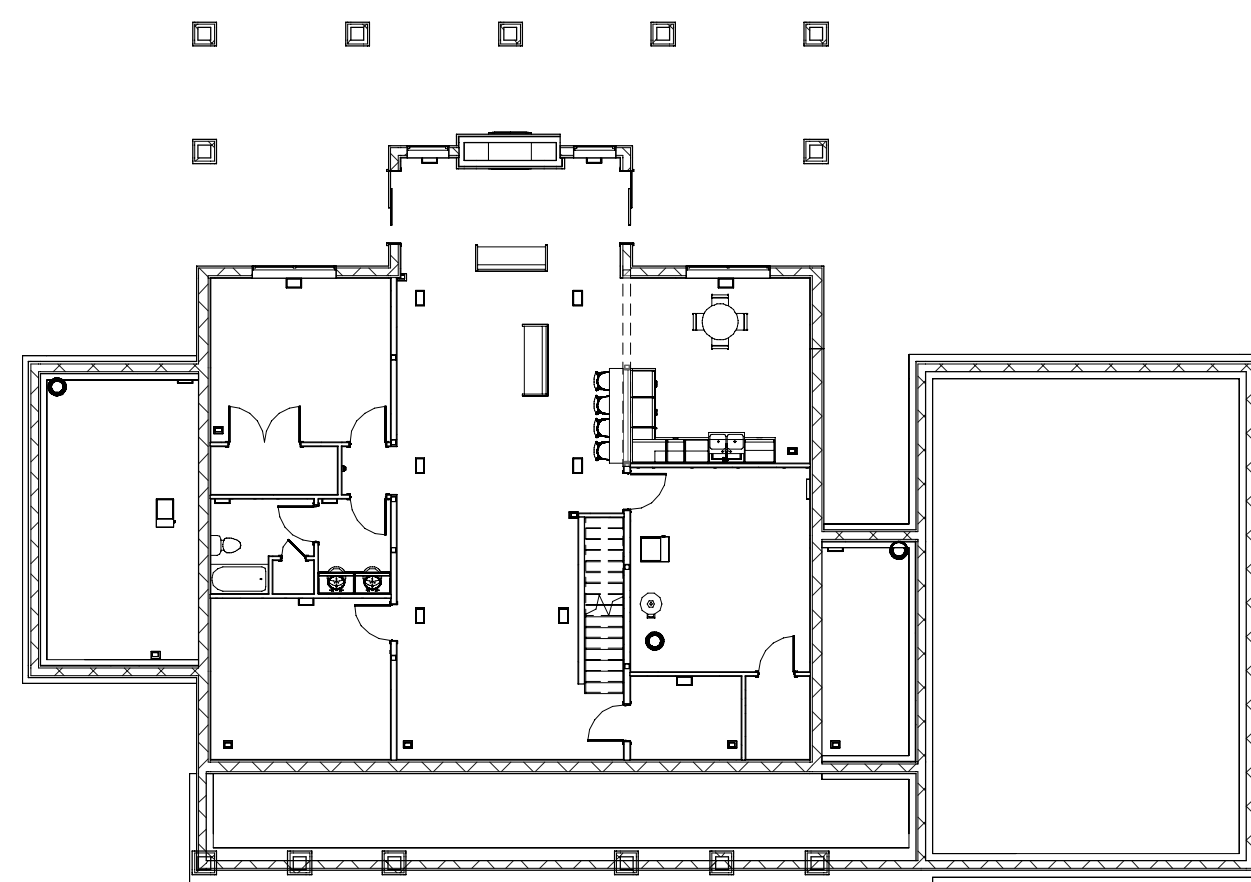
③ Basement 1/16" = 1'-0"
