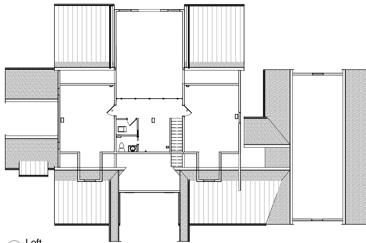
② Loft 1/16" = 1'-0"
