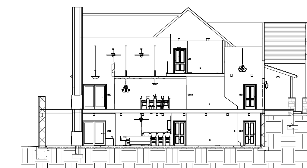
⑨ Section 2 1/16" = 1'-0"
