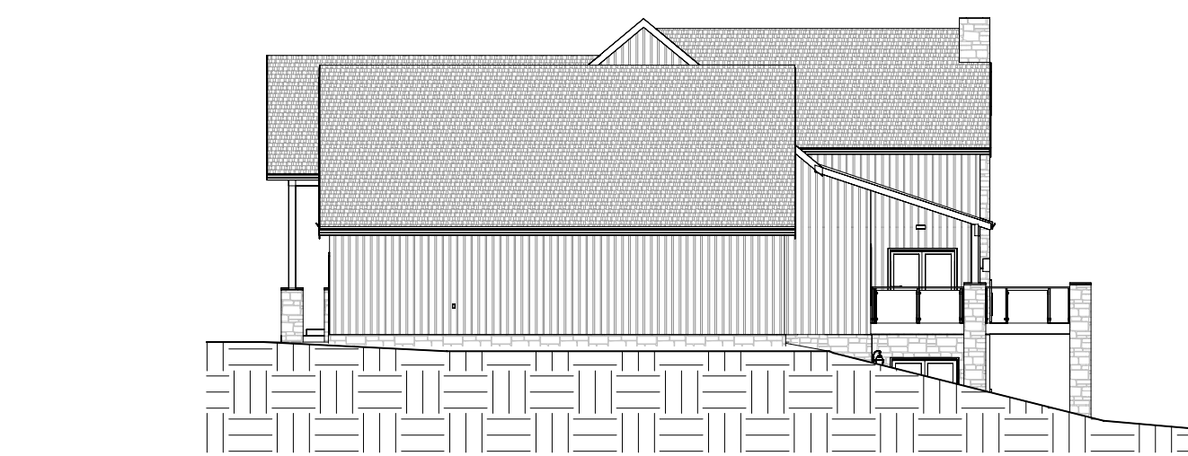
④ East 1/16" = 1'-0"
