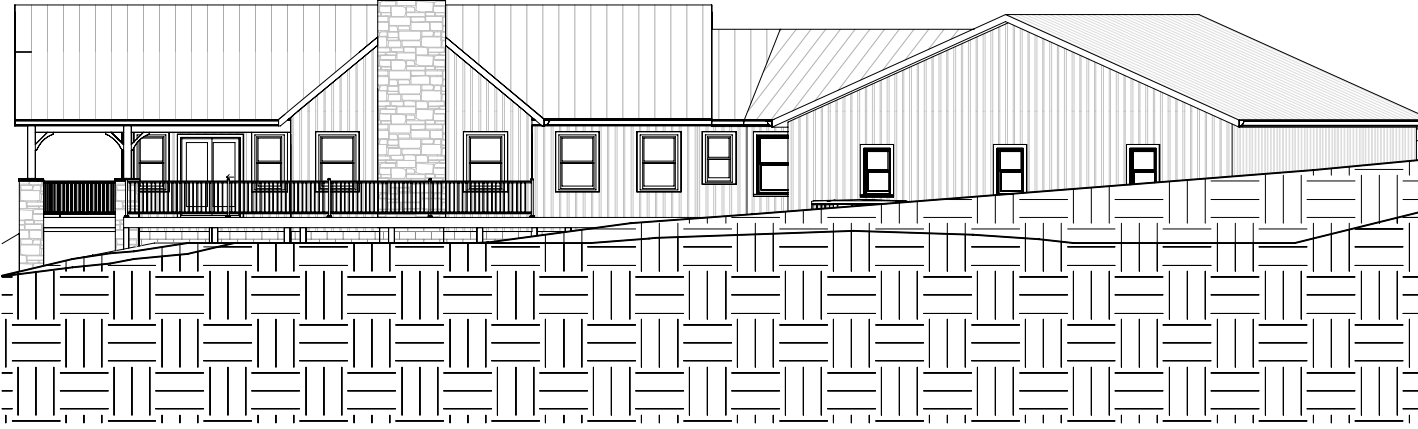
④ Elevation 2 - a 1/16" = 1'-0"
