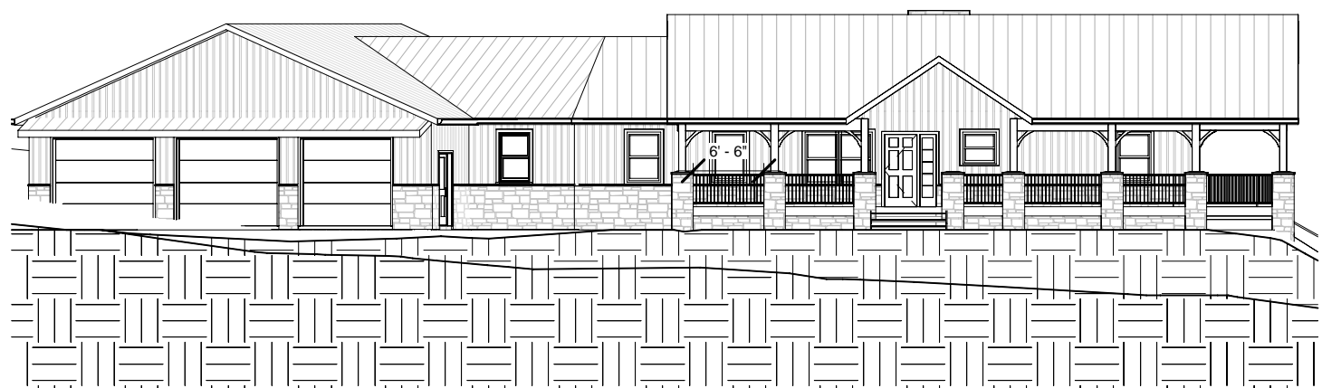
⑥ Elevation 4 - a 1/16" = 1'-0"
