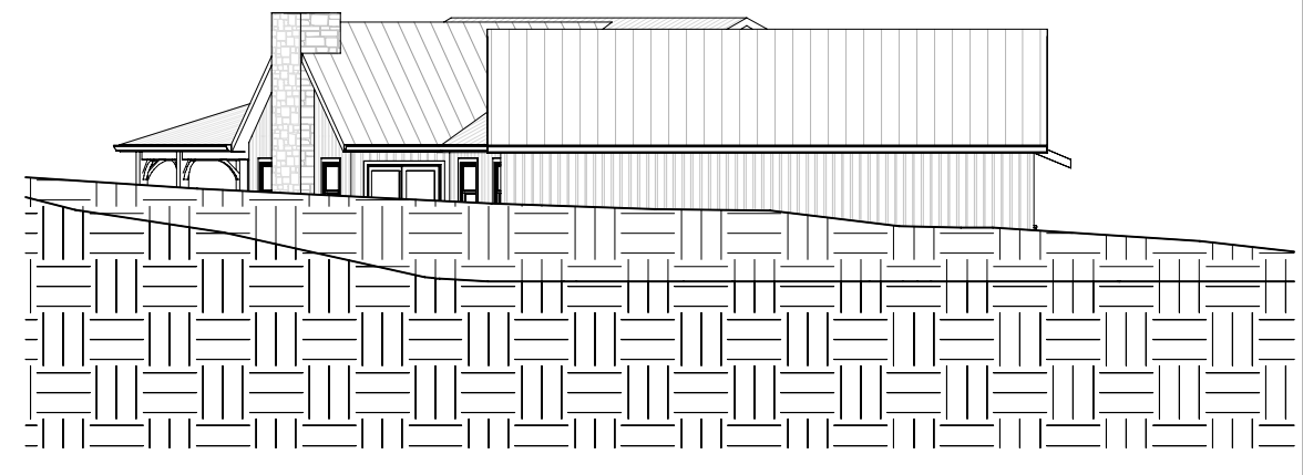
⑧ Elevation 6 - a 1/16" = 1'-0"
