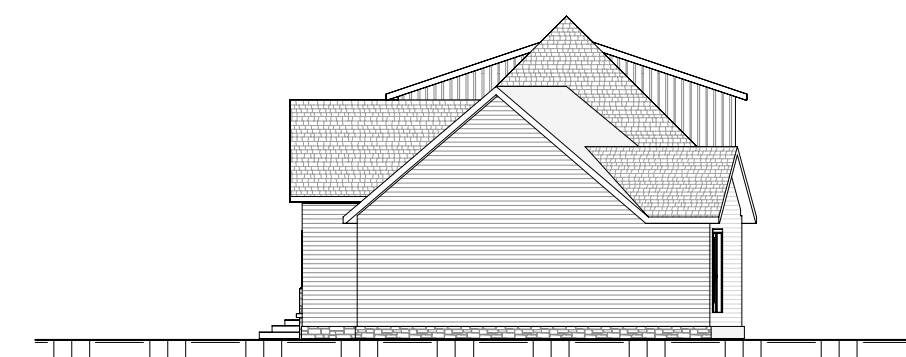
⑤ Elevation 3 1/16" = 1'-0"
