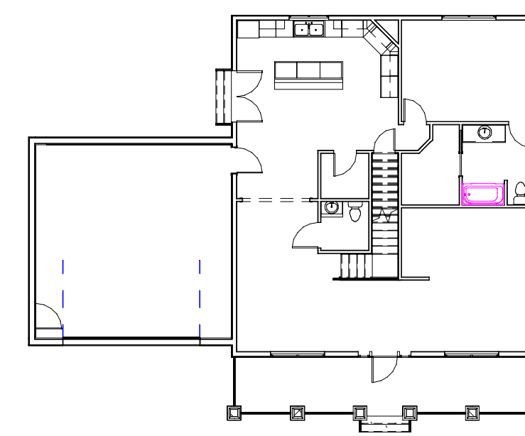
① New First Floor 1/16" = 1'-0"
