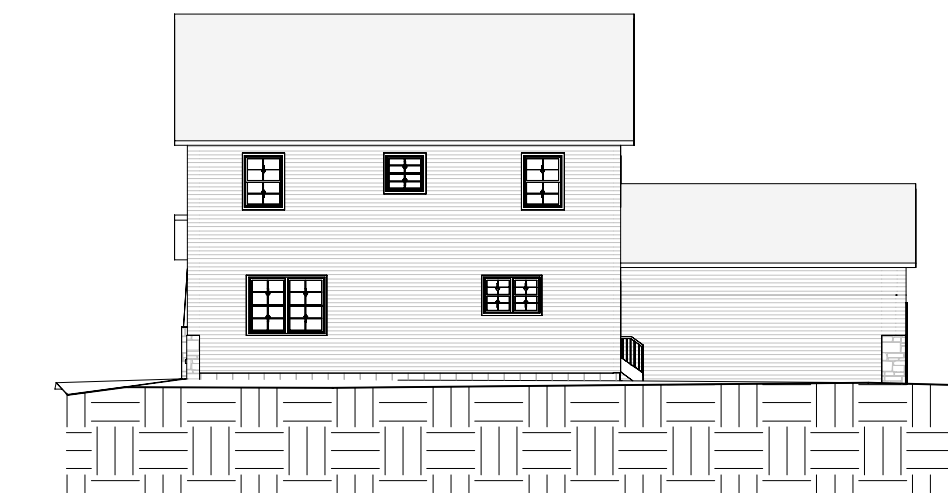
④ North 1/16" = 1'-0"
