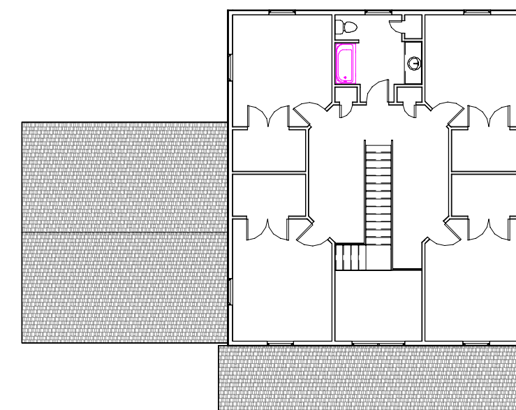
② New Second Floor 1/16" = 1'-0"
