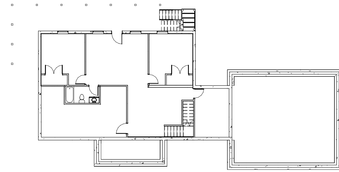
1 Basement 1/16" = 1'-0"
