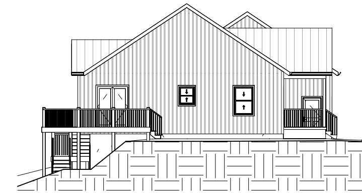
6 West 1/16" = 1'-0"
