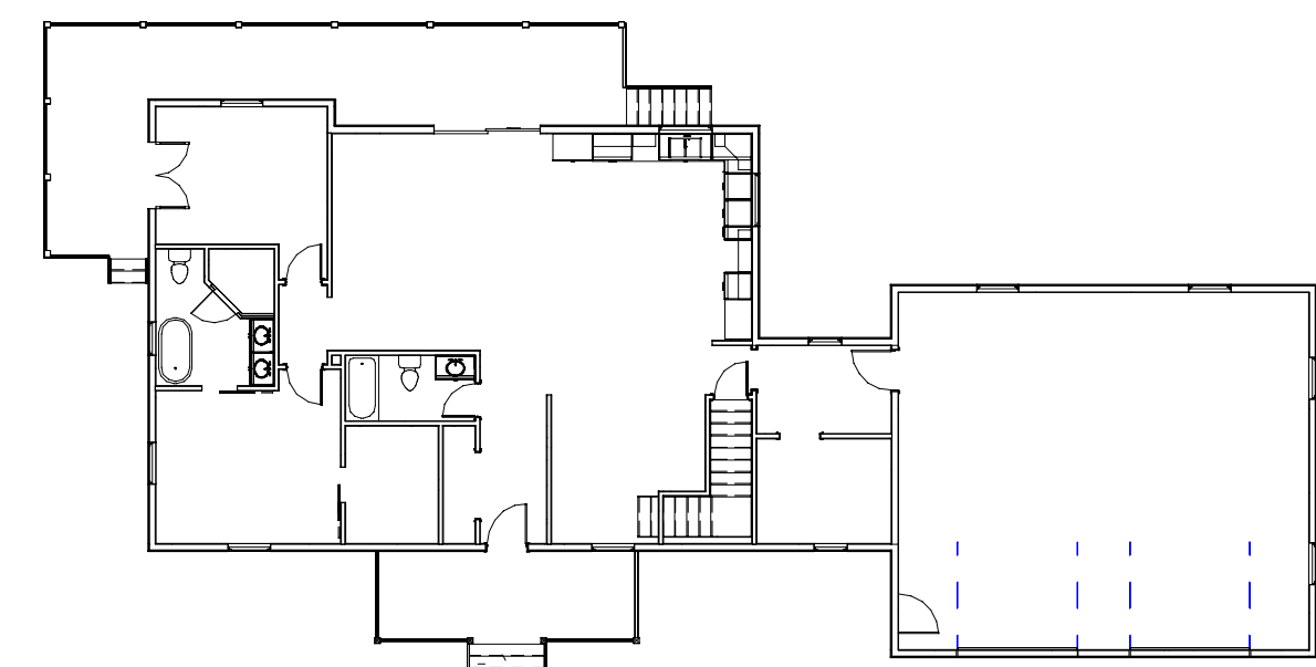
2 First Floor 1/16" = 1'-0"
