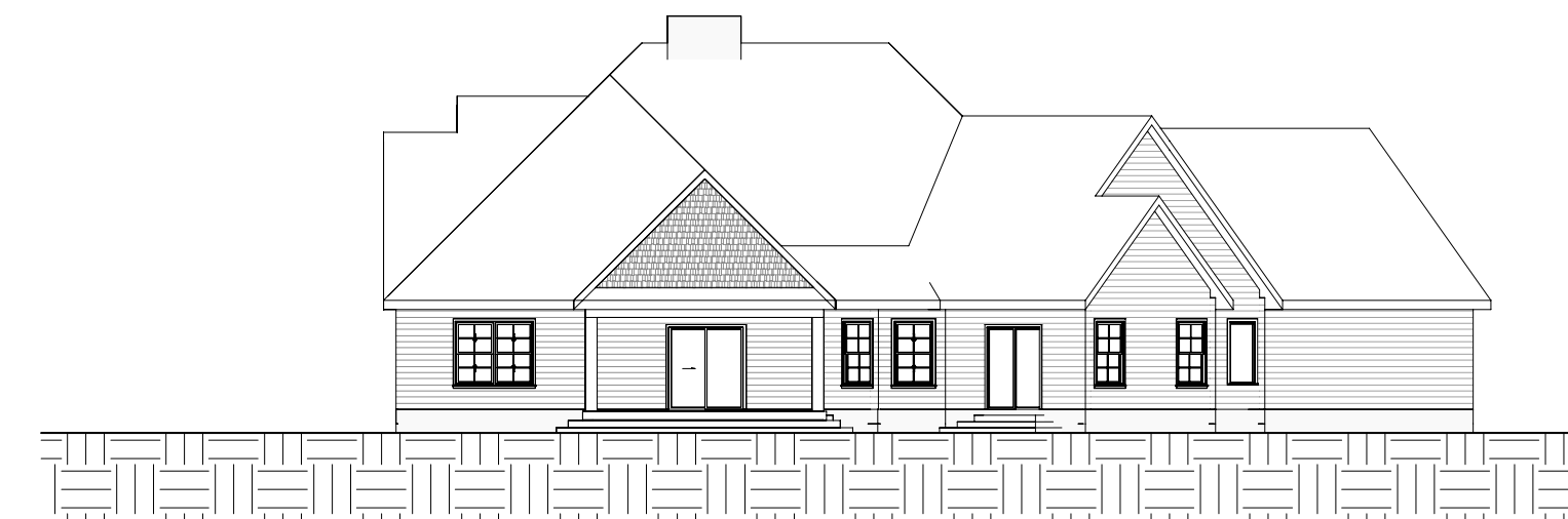
④ North 1/16" = 1'-0"
