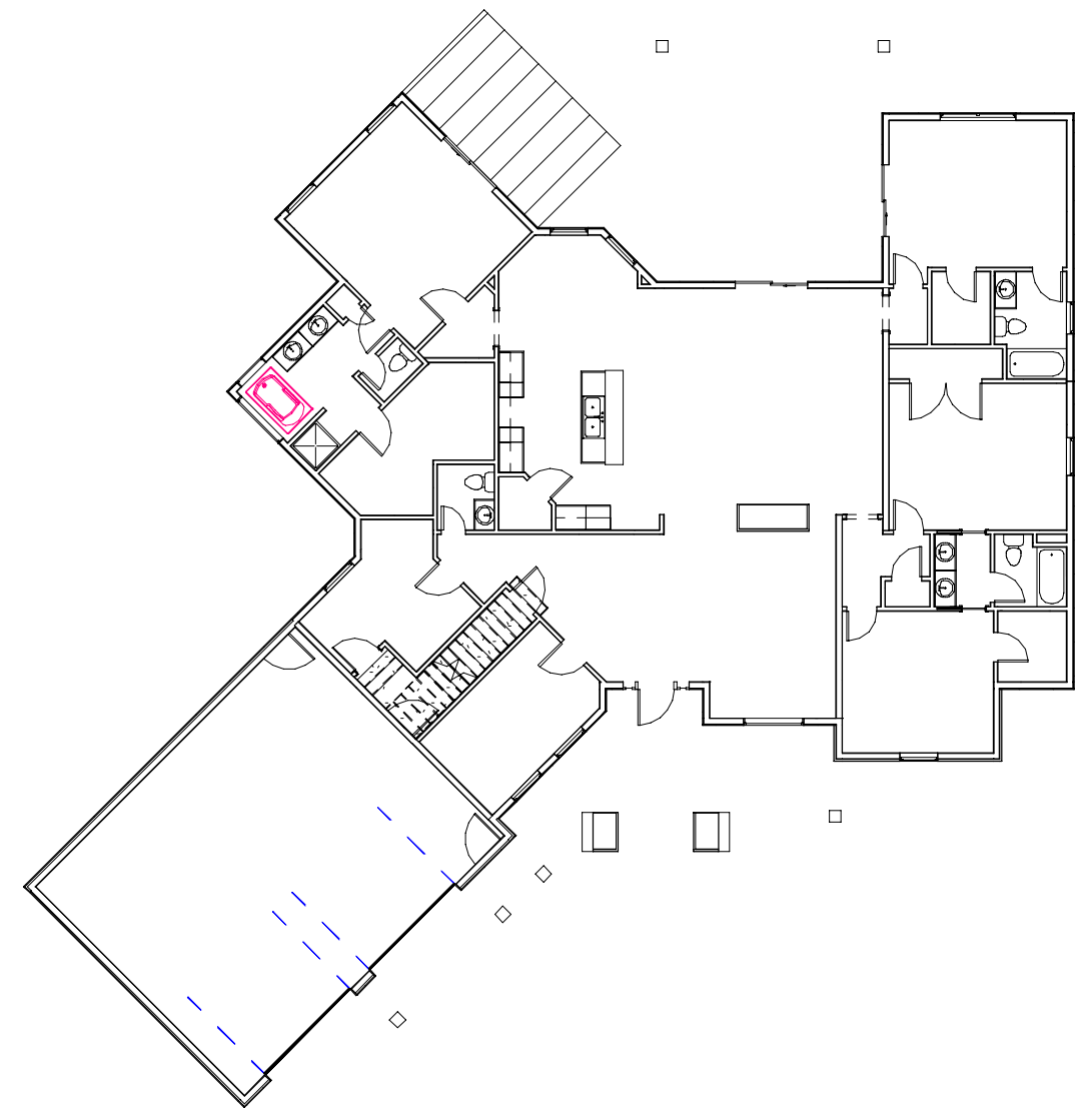
① First Floor 1/16" = 1'-0"
