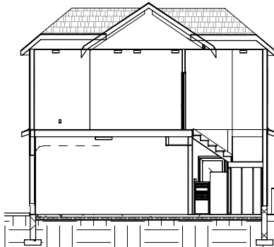
⑦ Section 1 1/16" = 1'-0'
