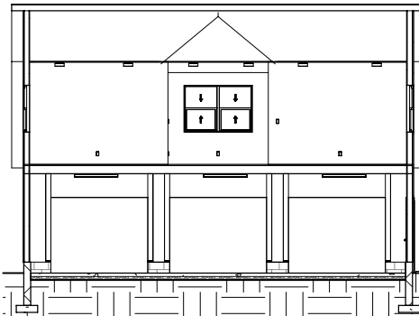
10 Section 4 1/16" = 1'-0'
