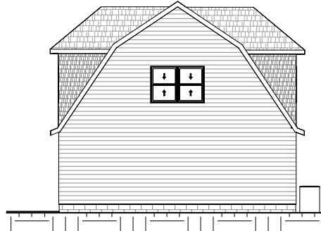
⑥ West 1/16" = 1'-0"
