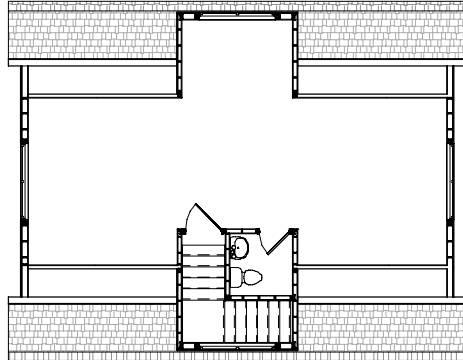
② Second Floor 1/16" = 1'-0"
