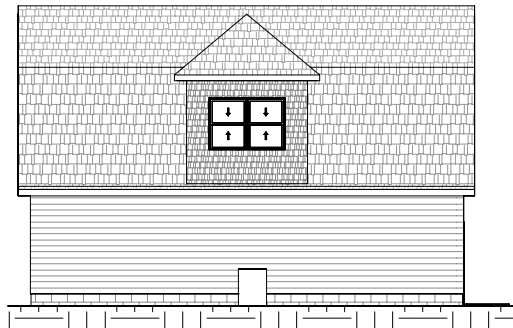
⑤ South 1/16" = 1'-0"
