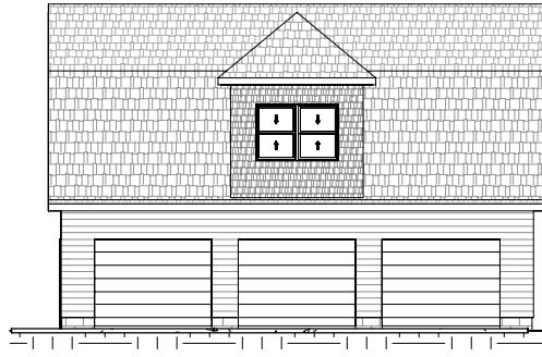
④ North 1/16" = 1'-0"
