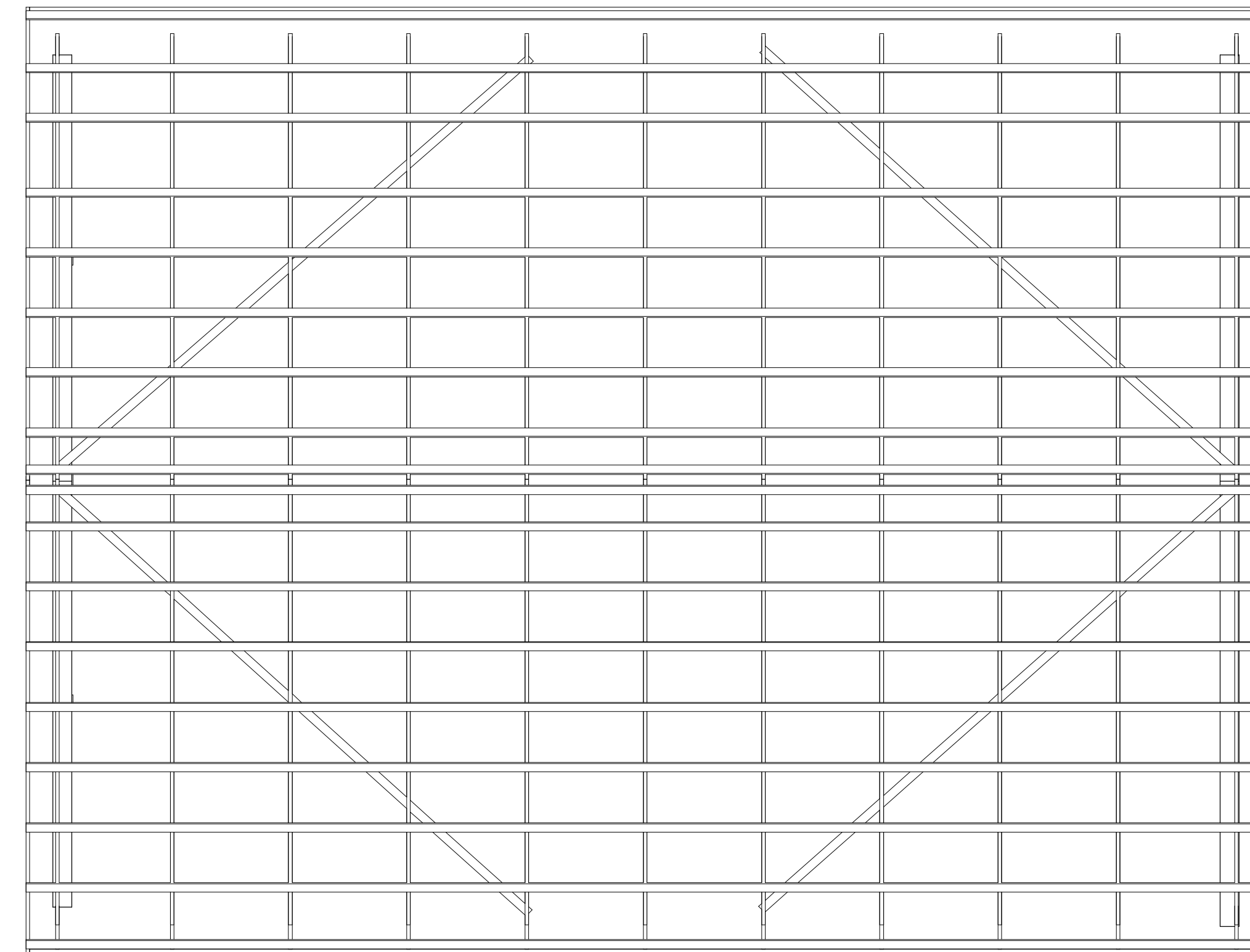
② Roof Framing Plan 1/4" = 1'-0"
