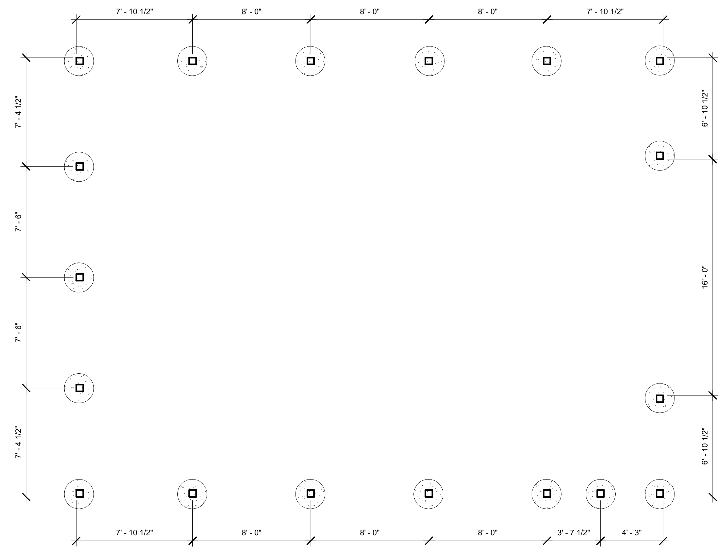
② Foundation Plan 1/4" = 1'-0"
